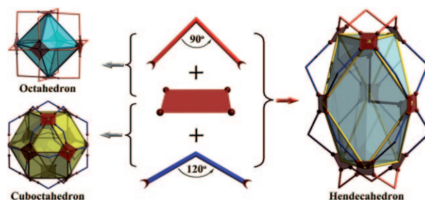
Figure 1. The self-assembly of three metal–organic polyhedra with ditopic angular linkers and four-connected square nodes.
