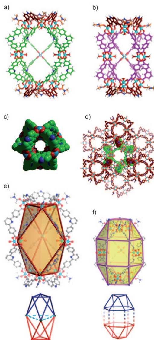
Figure 2. a,b) The molecular structures of 1 and 2 , respectively (Cu cyan; O red; N blue; C maroon, green, orange, or pink; H white). c) Space-filling representation of 1 viewed from the [001] direction. d) Molecular packing of 1 in the crystal structure with space-filling representation highlighting the intermolecular \pi – \pi interactions. e,f) Schematic representation of the polyhedra when considering the metal clusters or ligands, respectively, as vertices.
