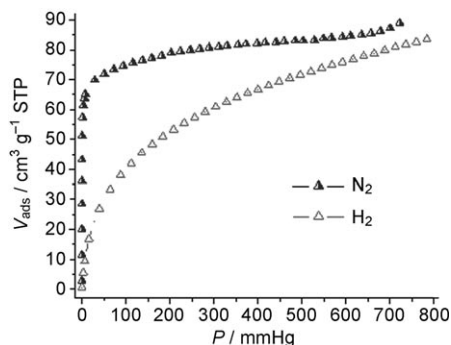
Figure 3. N 2 and H 2 adsorption isotherms of 1 at 77 K.
